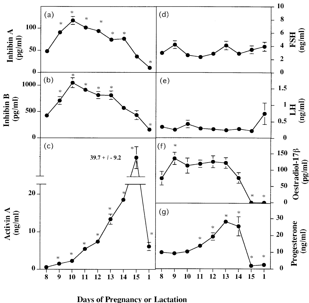
Figure 2 Changes in plasma concentrations of (a) inhibin A, (b) inhibin B, (c) activin A, (d) FSH, (e) LH, (f) oestradiol-17 \beta and (g) progesterone during the second half of pregnancy and in early lactation in the golden hamster. Each value represents the mean \pm S.E.M. of five animals. * P < 0.05 compared with the value at day 8 of pregnancy (Duncan's Multiple Range test for inhibin A, inhibin B, FSH, LH and oestradiol-17 \beta ; Student's t -test for activin A and progesterone).
