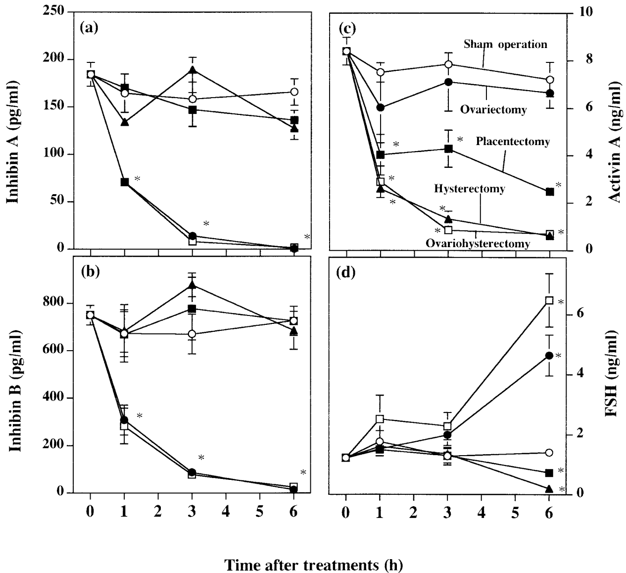
Figure 3 Plasma concentrations of (a) inhibin A, (b) inhibin B, (c) activin A and (d) FSH after ovariectomy (●), placentectomy (■), hysterectomy (▲), ovari hysterectomy (□) or sham operation (○) at 1100 h on day 12 of pregnancy in the golden hamster. Each value represents the mean \pm S.E.M. of five observations. * P < 0.05 , significantly different from time-matched sham-operated group (Student's t -test for inhibin A and activin A; Duncan's New Multiple Range test for inhibin B and FSH).
