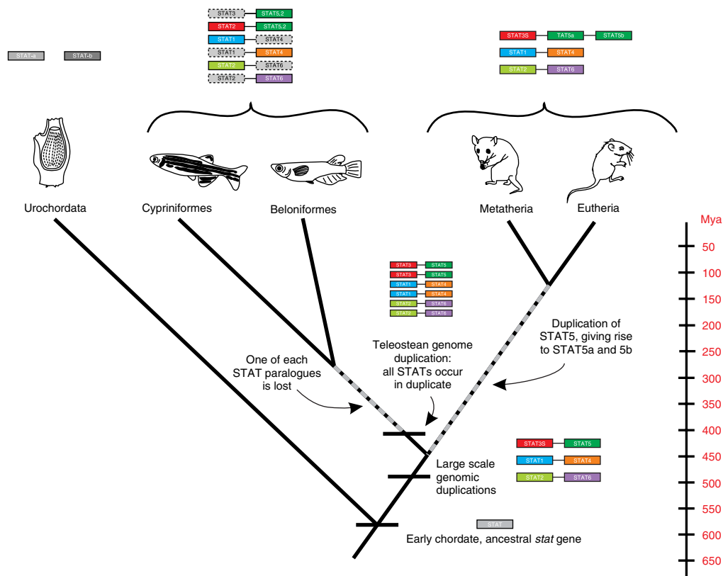
Figure 6 A proposed mechanism for STAT evolution: including 2R hypothesis as a basis of the radiation of the stat repertoire, the fish-specific whole genome duplication (3R), and subsequent (partial) loss of paralogous stat genes. Animal diagrams from left to right: sea squirt ( Ciona intestinalis ), zebrafish ( Danio rerio ), Japanese medaka ( Oryzias latipes ), opossum ( Monodelphis domestica ), and mouse ( Mus musculus ).
