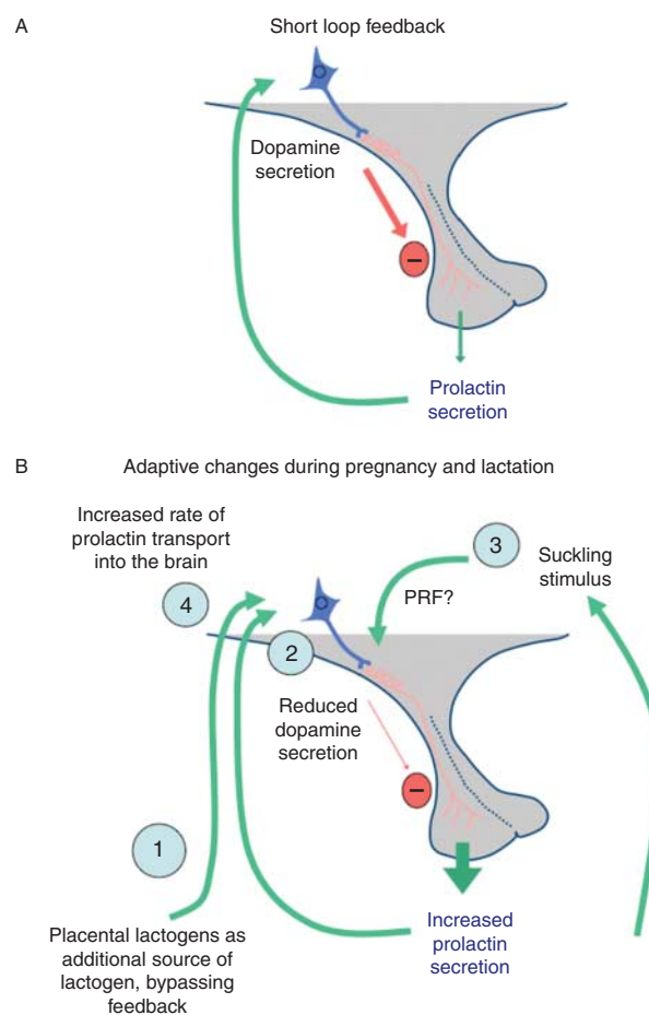
Figure 2 (A) Diagrammatic representation of short loop feedback control of prolactin secretion. (B) Adaptive changes in the regulation of prolactin secretion during pregnancy and lactation. Note that there are multiple adaptive processes to ensure elevated levels of lactogenic hormones present both in the blood and in the brain of the mother, potentially regulating a wide range of functions to facilitate lactation: 1) Production of prolactin-like molecules from the placenta to bypass feedback regulation of pituitary prolactin secretion. 2) Plasticity in the TIDA neuronal response to prolactin, with reduced secretion of dopamine and induction of enkephalin expression. 3) Maternal behavioural adaptation to suckle the pups, providing the most powerful prolactin-releasing stimulus known. 4) Increased transport of prolactin into the brain during lactation.
